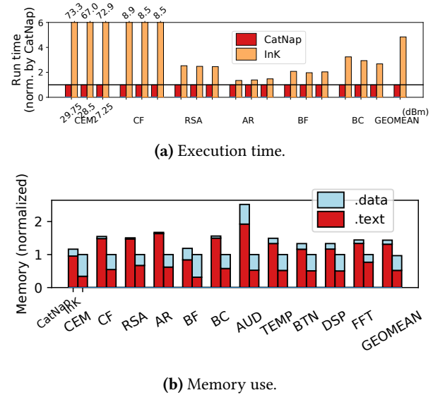
Figure 7. Performance and memory use of CatNap.
