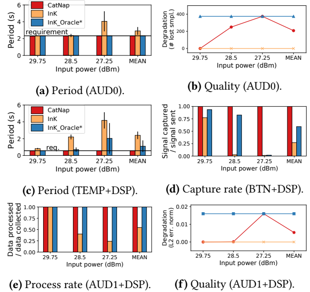
Figure 6. Result of different benchmarks. The (a) period and (b) quality for AUD0, the (c) period of TEMP+DSP, the (d) capture rate of BTN+DSP, and the (e) portion of processed data and the (f) quality for AUD1+DSP is shown. User-specified requirement is shown as a horizontal line (a, c). *InK_Oracle was manually tuned for best performance.
