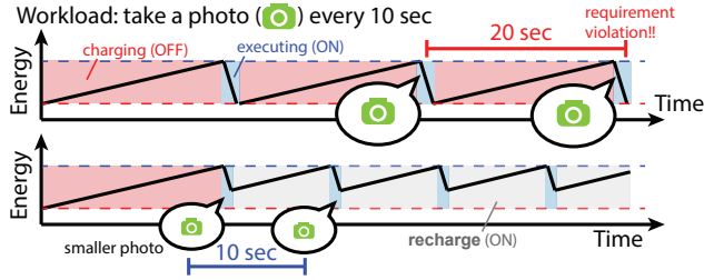
Figure 1. Periodic execution. Attempts to periodically take a photo (shaded blue) every 10 seconds is shown. Periodic execution fails with low power (top) because the charging time (shaded red) necessary to take a photo exceeds the desired period of 10 seconds. With degradation (bottom), the periodic requirement is met by the system deciding to start recharging early (shaded gray) after taking a smaller photo.
