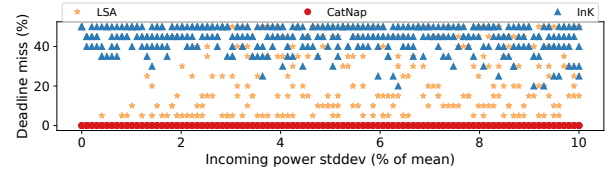
(a) Deadlines missed with short-term power fluctuation (C2). The figure shows deadlines missed as power fluctuation increases for LSA, InK, and CatNap.
